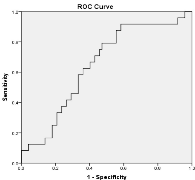
Figure 1. ROC analysis to determine NLR cut-off value
